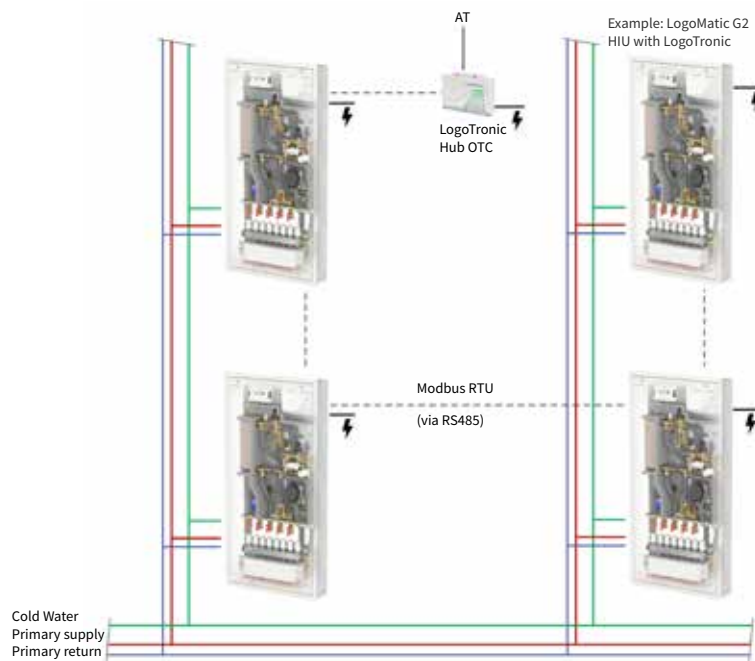
Fig. 1: LogoTronic Hub OTC in the system integration with several LogoMatic G2 Heat Interface Units.
